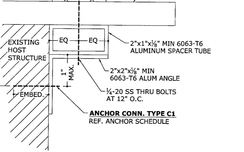
4 5 N.T.S. VERT SECTION PASS THRU WINDOW DETAIL
