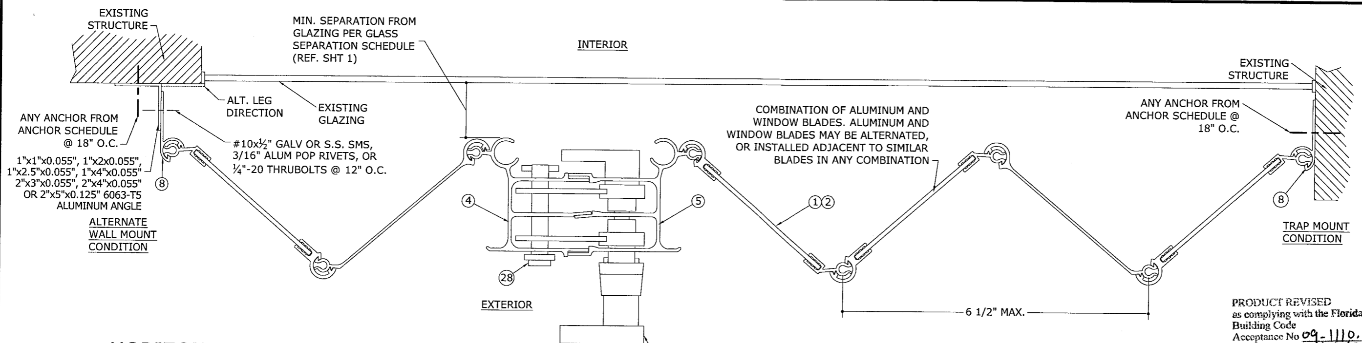
1 5 N.T.S. HORIZ SECTION HORIZONTAL SECTION W/ COMBINATION BLADES
