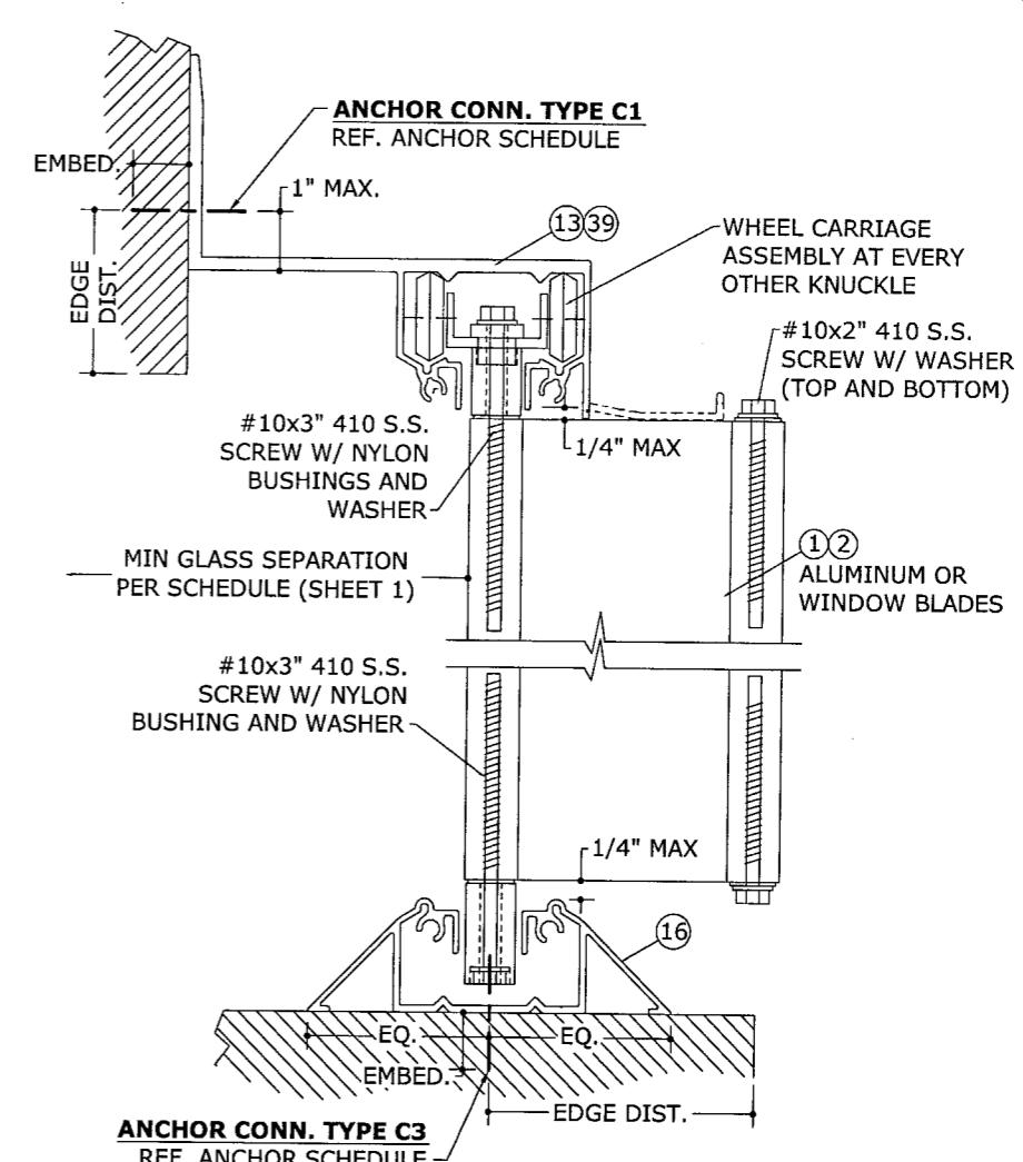
3 B.O. WALL HEADER 6 WALKOVER TRACK N.T.S. VERT SECTION
