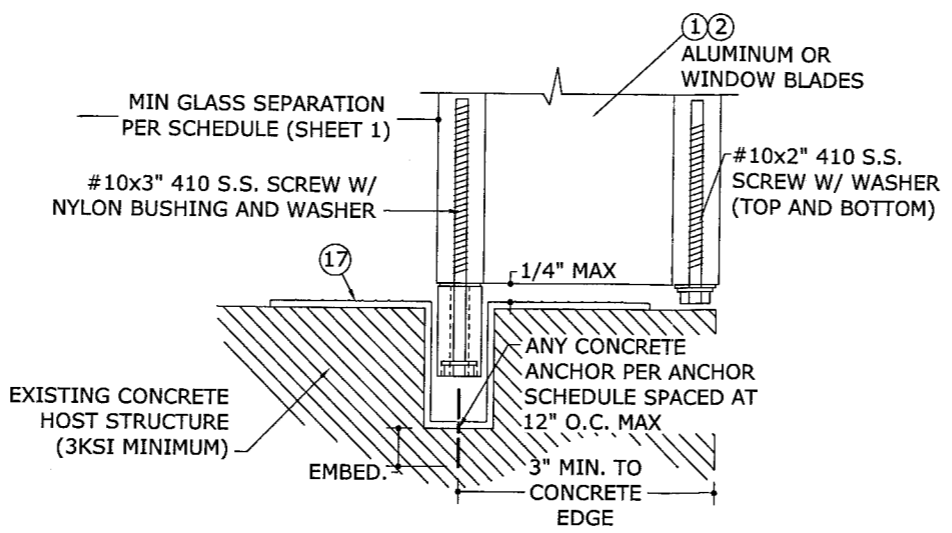
4 RECESSED FLOOR TRACK 6 N.T.S. VERT SECTION
