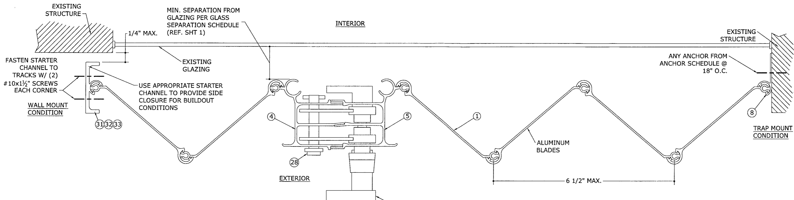
1 HORIZONTAL SECTION W/ ALUMINUM BLADES 4 N.T.S. HORIZ SECTION
