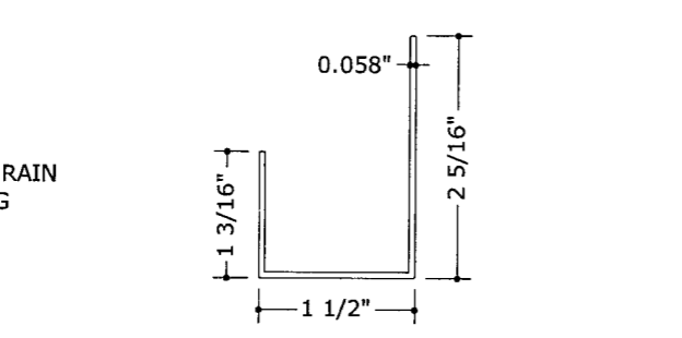
11 ADJUSTABLE SILL TRACK BOTTOM N.T.S. 6063-T6
