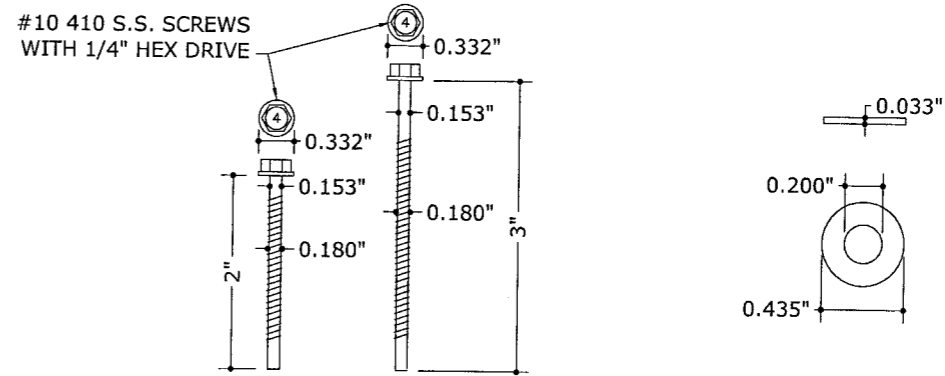
20 KNUCKLE SCREWS STAINLESS STEEL 21 WASHER N.T.S. STAINLESS STEEL
