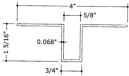
17 RECESSED TRACK N.T.S. 6063-T5
