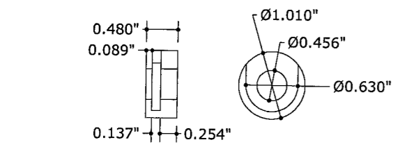
25 LEFT LOCKING ARM BUSHING N.T.S. NYLON
