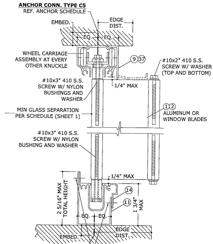
2 CEILING HEADER 6 ADJUSTABLE SILL TRACK N.T.S. VERT SECTION
