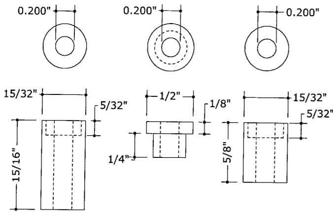
22 NYLON BUSHINGS N.T.S. NYLON
